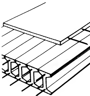
⑦ Prefabricated reinforced concrete I-beam floor
